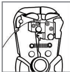
Tension Knob micro-adjust for wire 30 AWG (0.05 mm 2 )
